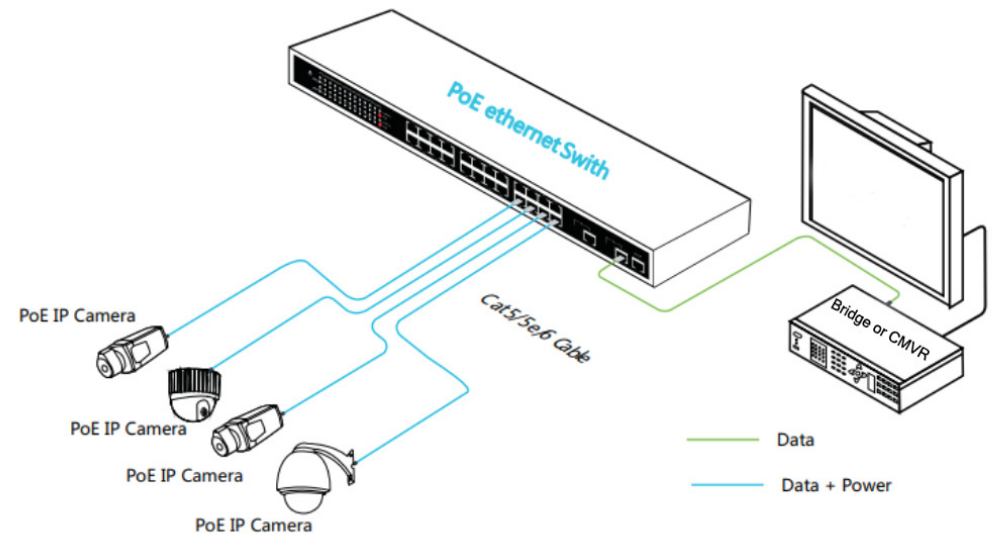
Figure 1: System Design
