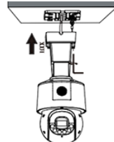
Ceiling bracket
